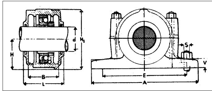
Plummer Blocks : Series S. 600 (Suitable for Brg. No. 1300, 2300, 22,300 Series)
